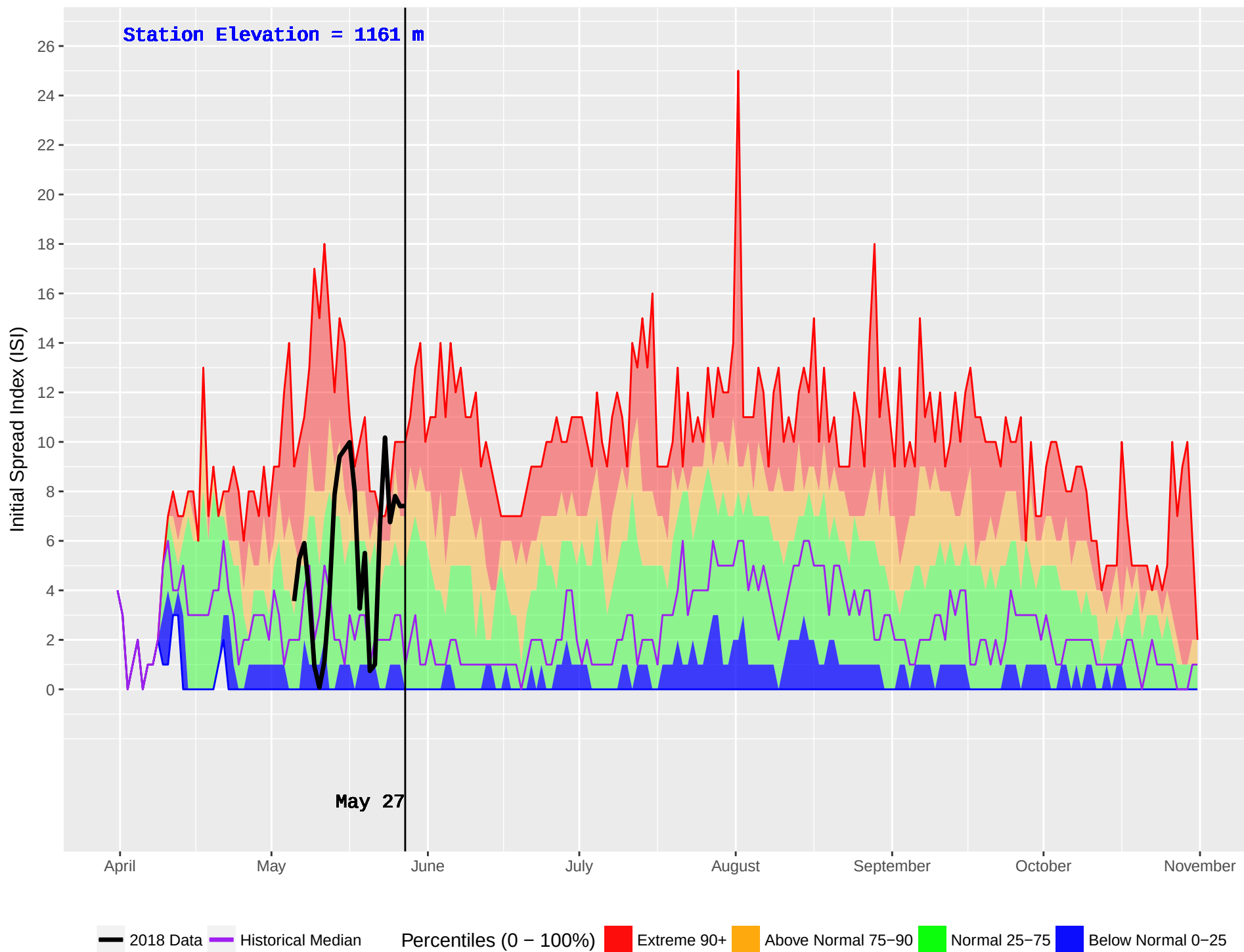
TIMOTHY (234) : Historical (1990–2016) and Current (2018) Noon Initial Spread Index (ISI)
