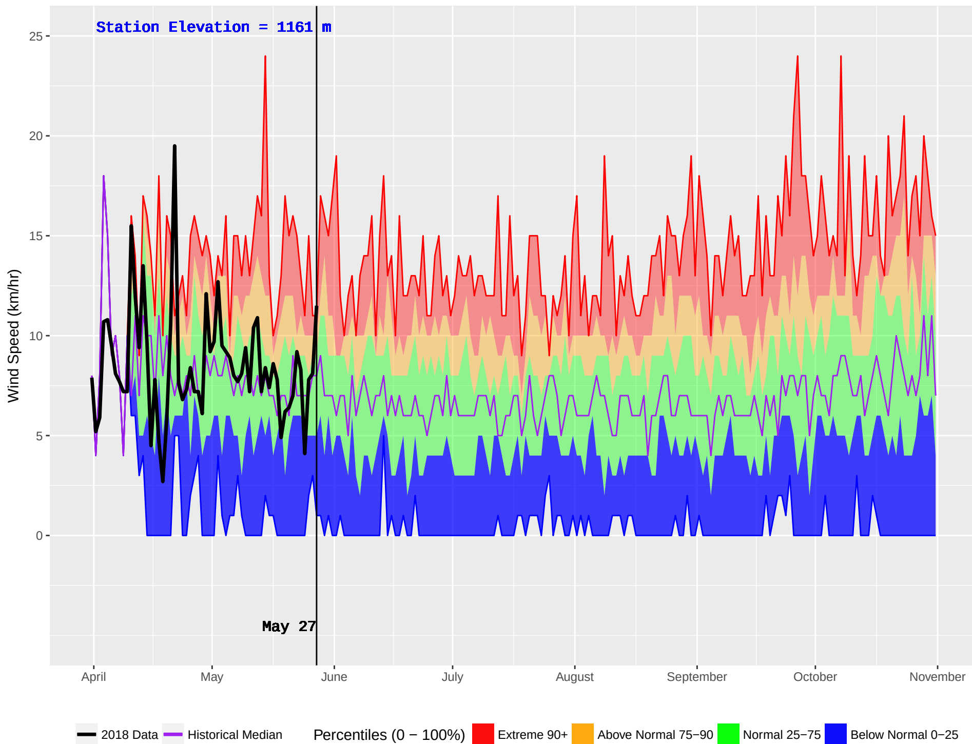
TIMOTHY (234) : Historical (1990–2016) and Current (2018) Noon Wind Speed
