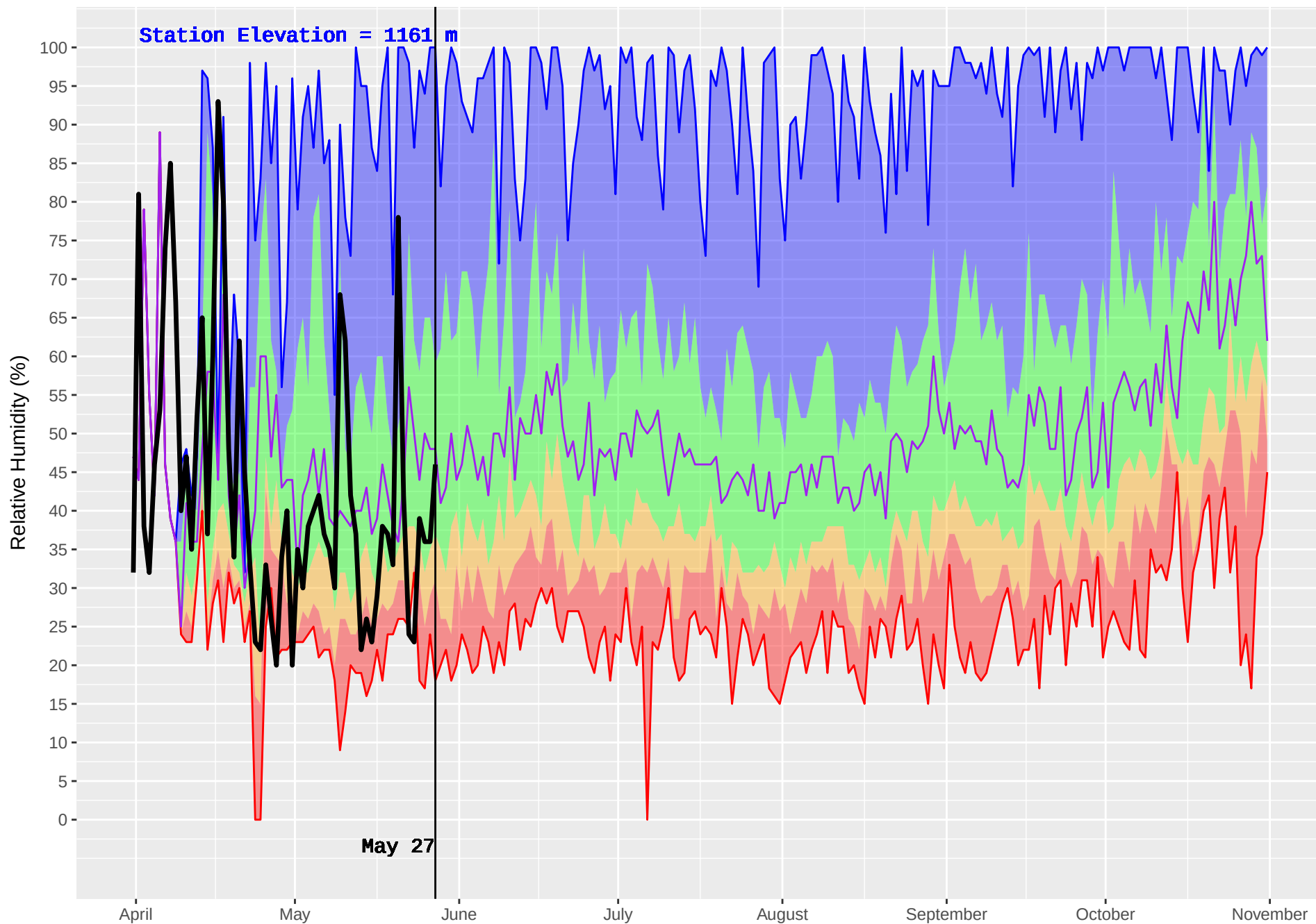
TIMOTHY (234) : Historical (1990–2016) and Current (2018) Noon Relative Humidity
