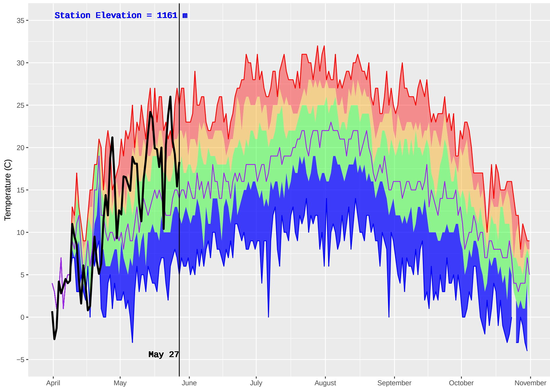
TIMOTHY (234) : Historical (1990–2016) and Current (2018) Noon Temperature
