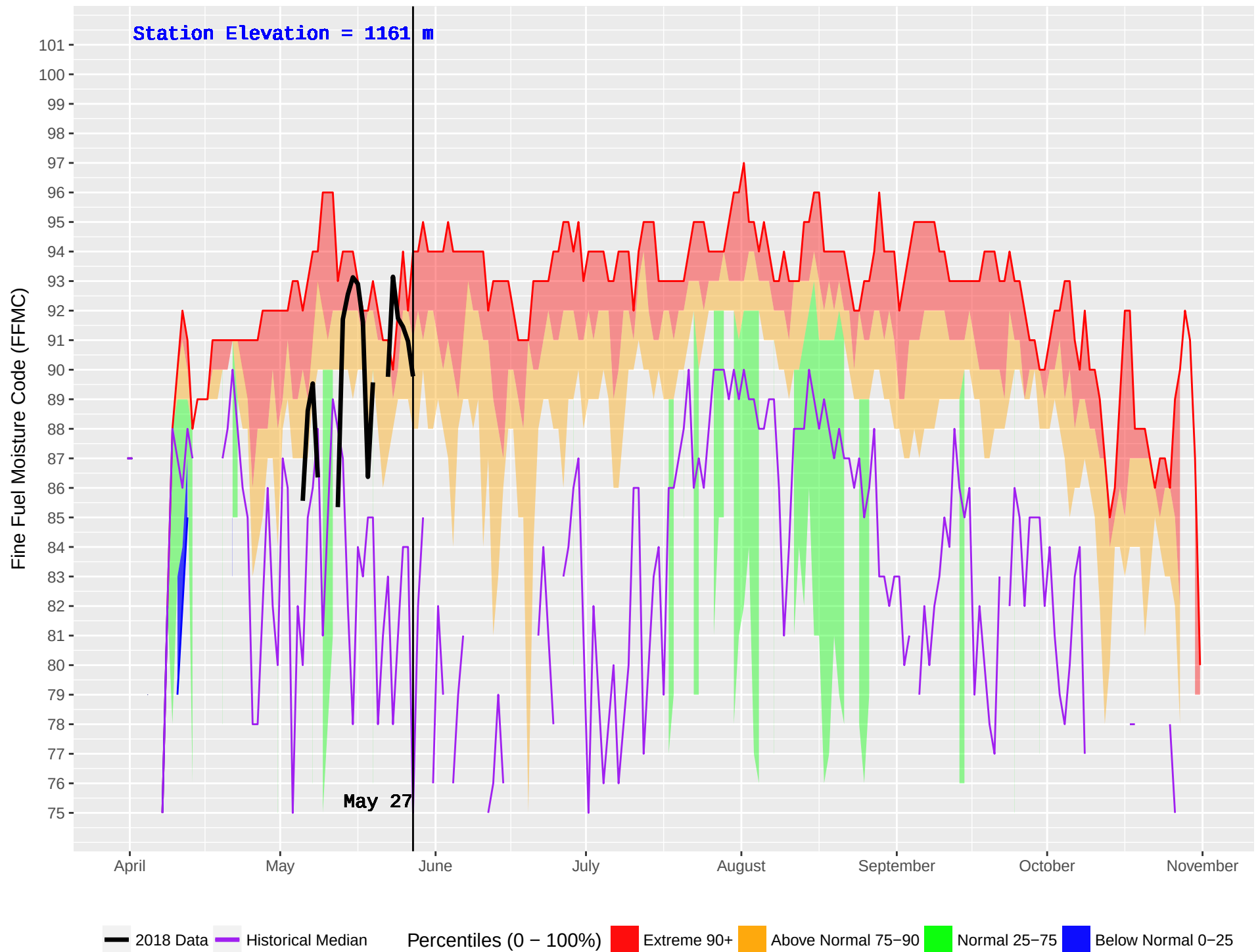
TIMOTHY (234) : Historical (1990–2016) and Current (2018) Noon Fine Fuel Moisture Code (FFMC)
