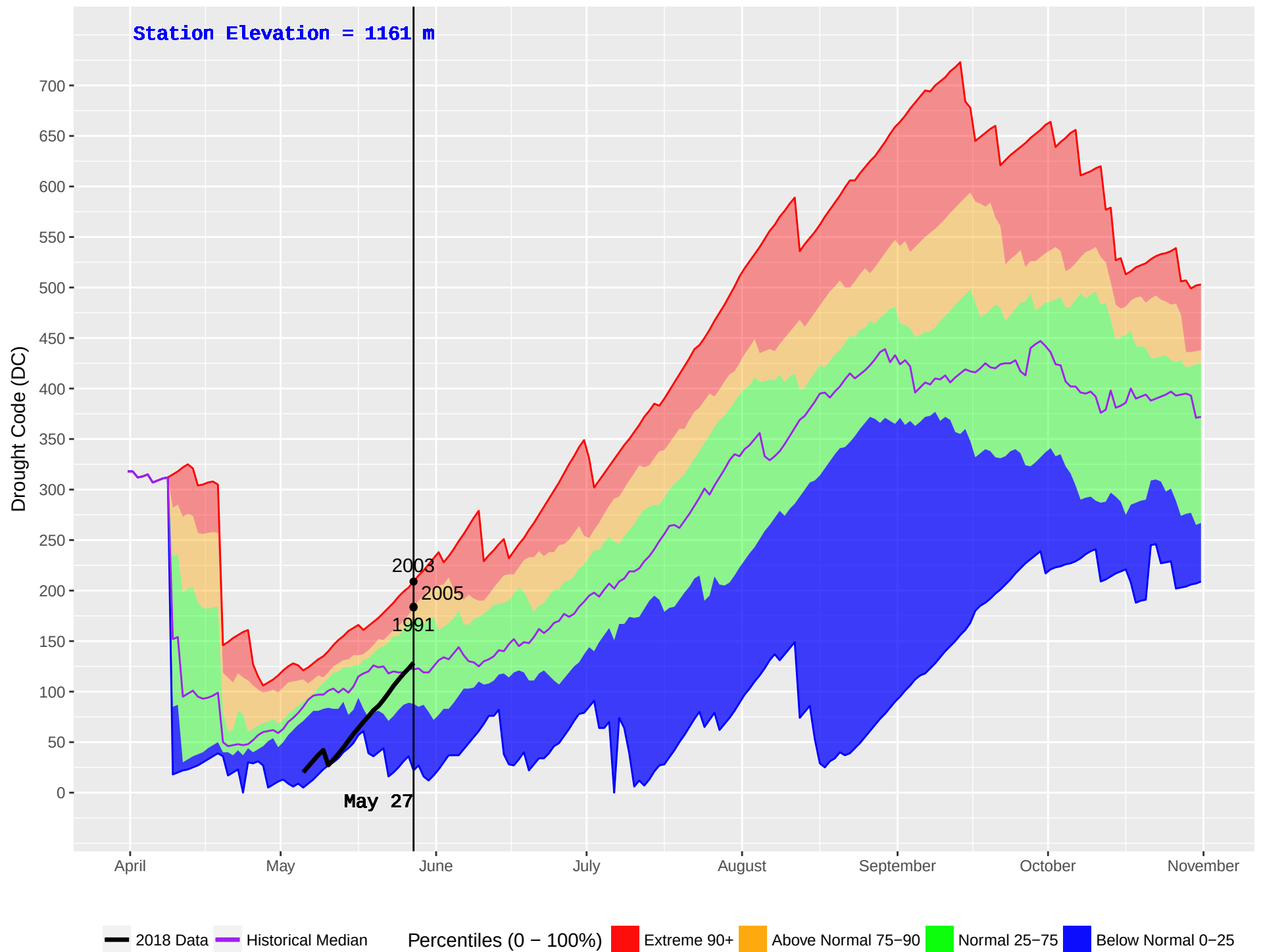
TIMOTHY (234) : Historical (1990–2016) and Current (2018) Noon Drought Code (DC)
