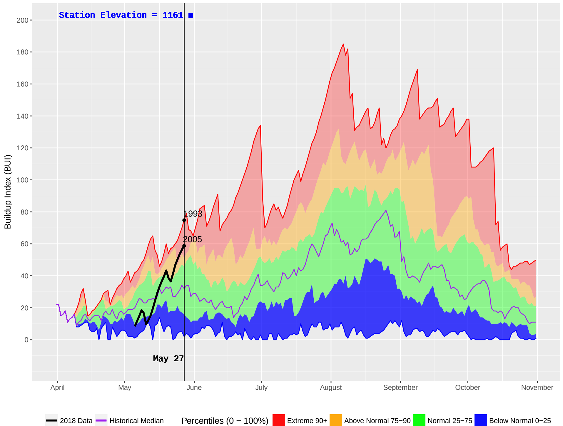
TIMOTHY (234) : Historical (1990–2016) and Current (2018) Noon Buildup Index (BUI)
