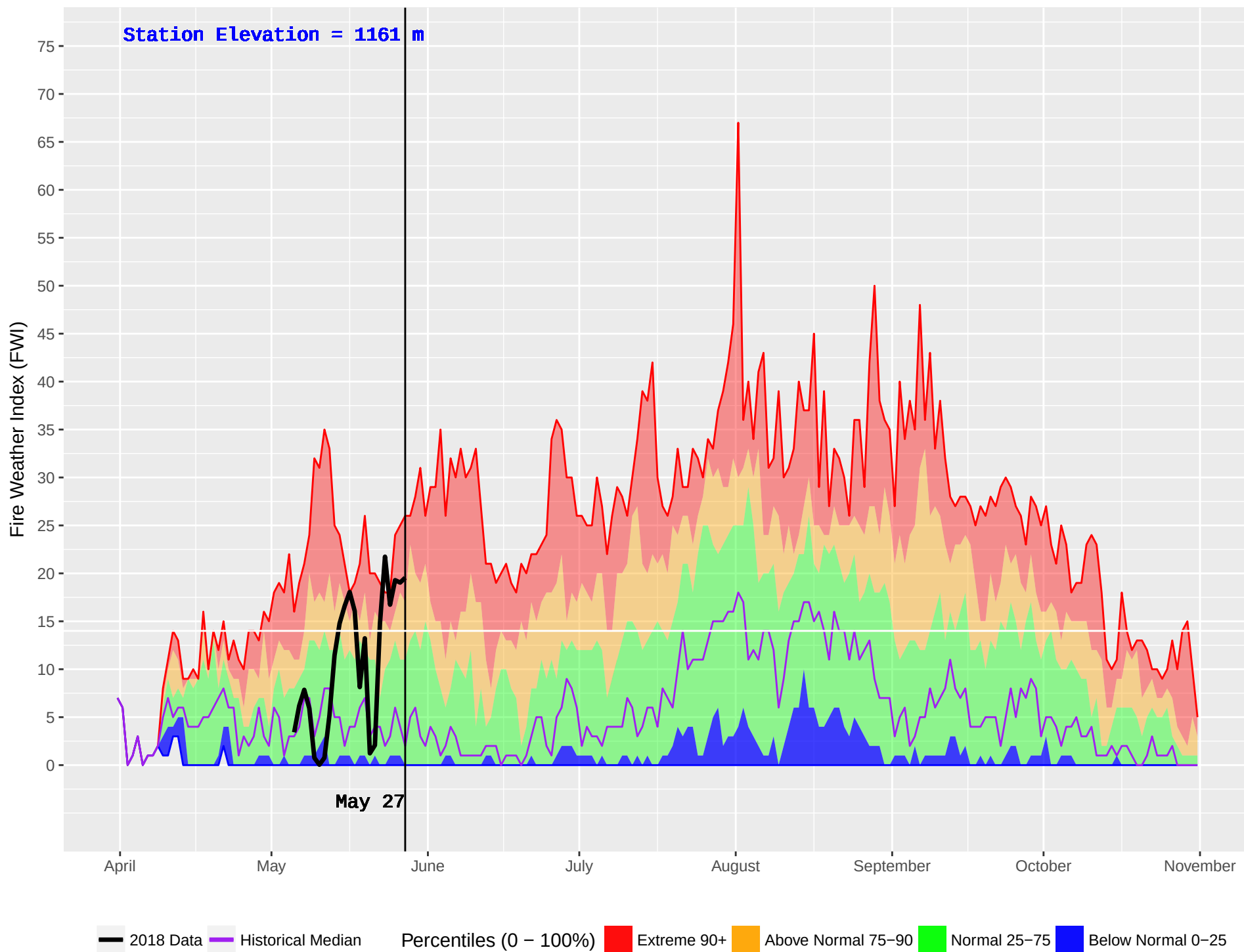
TIMOTHY (234) : Historical (1990–2016) and Current (2018) Noon Fire Weather Index (FWI)
