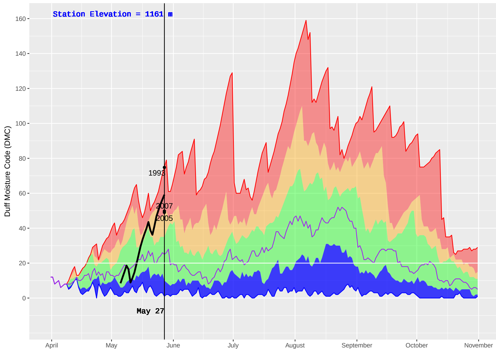
TIMOTHY (234) : Historical (1990–2016) and Current (2018) Noon Duff Moisture Code (DMC)
